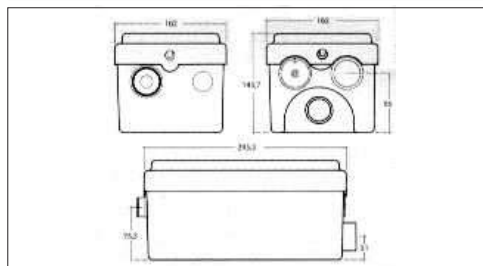
SANISHOWER Plato ducha+lavabo
