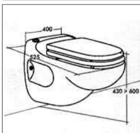
COMPACT STAR wc+lavabo
