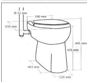
COMPACT 43 wc+lavabo
